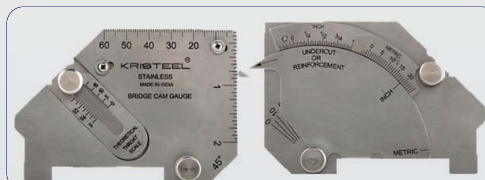
UNIVERSAL WELDING GAGE
